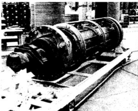
HERCULES airframe begins to take shape when machined and painted castings are placed on assembly fixture (left). After skin panels are riveted on, workers enter main engine section to shoot silastic sealant into seams (right).
