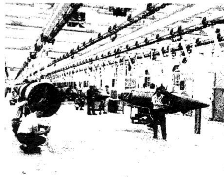
FINISHED airframe sections (left) are hoisted onto overhead monorail for final assembly. As sections move along hairpin-shaped course, workers install internal mechanisms and insert cable harness for the guidance and control package (right).
