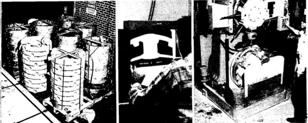
ROUGH aluminum and magnesium castings (left), trucked to Douglas from subcontractors in New York, New Jersey and Pennsylvania, are checked for flaws with X-ray unit. After large diameters are machined on vertical turret lathe, castings are drilled and tapped (right).
