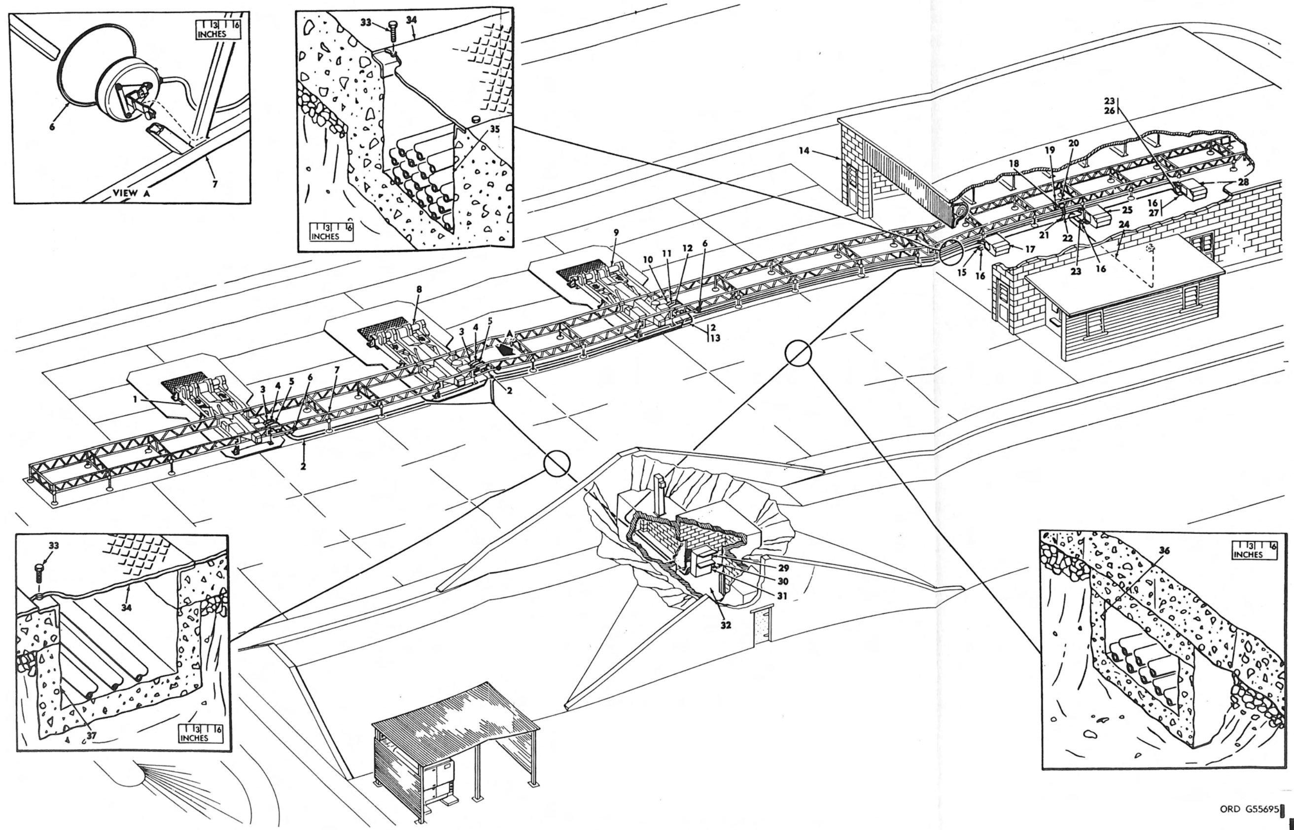
Figure 289.28. Hercules USAREUR launching section—cable assembly locations—removal and installation.
