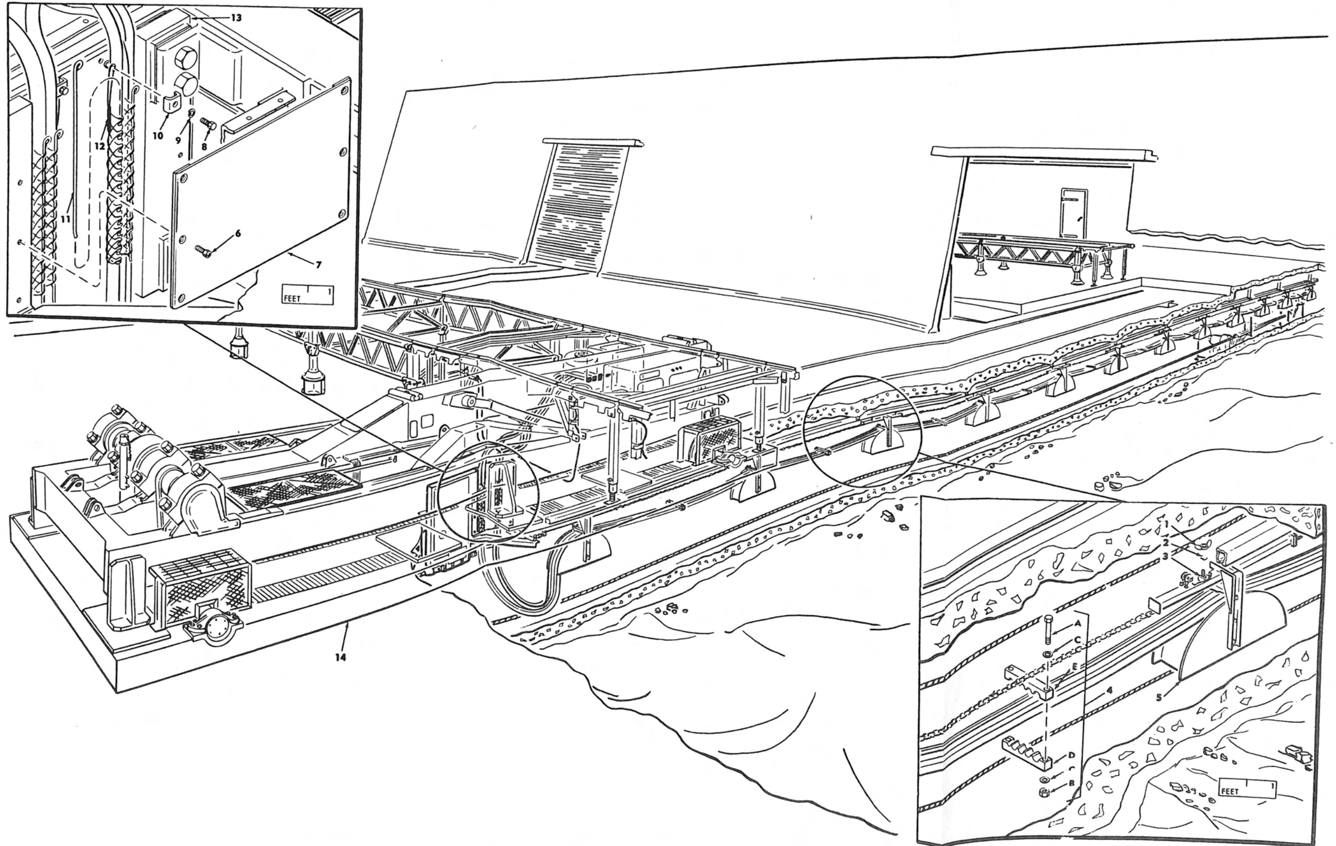
Figure 289.21. Hercules USARAL cable assemblies—removal and installation—typical for Hercules monorail launcher assemblies No. 1 and No. 2.
