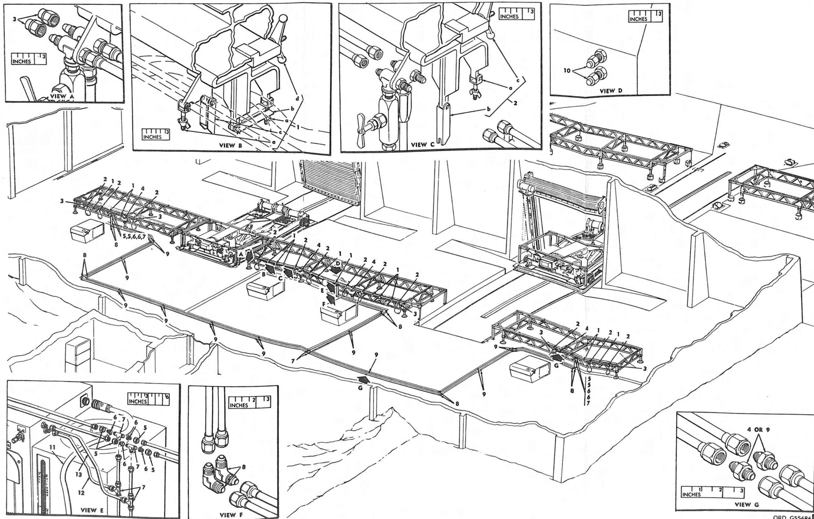
Figure 289.19. Hercules USARAL launching section modification kit hydraulic system—removal and installation.
