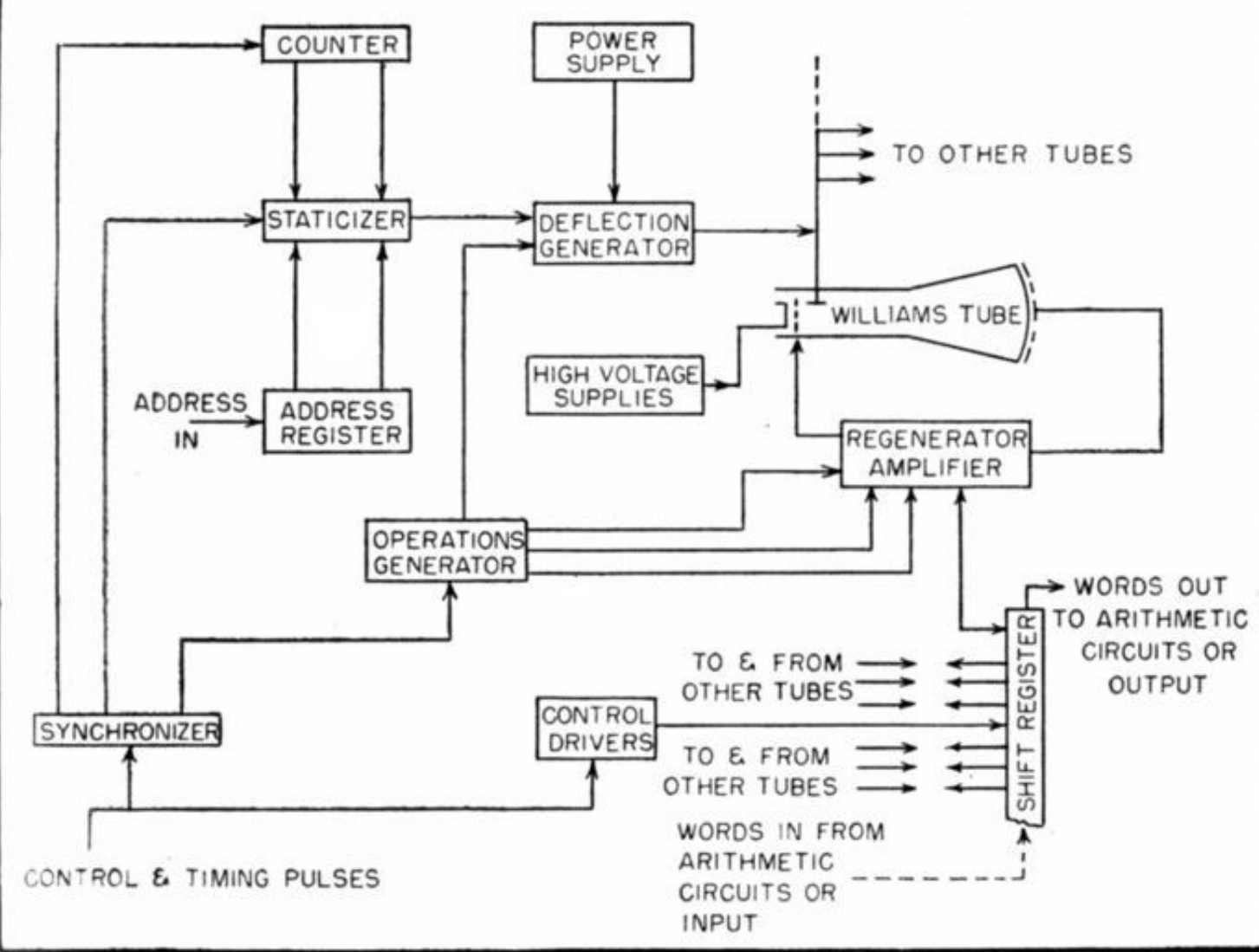
FIG. 5—Block diagram of electrostatic memory system using modified conventional cathode-ray tube
