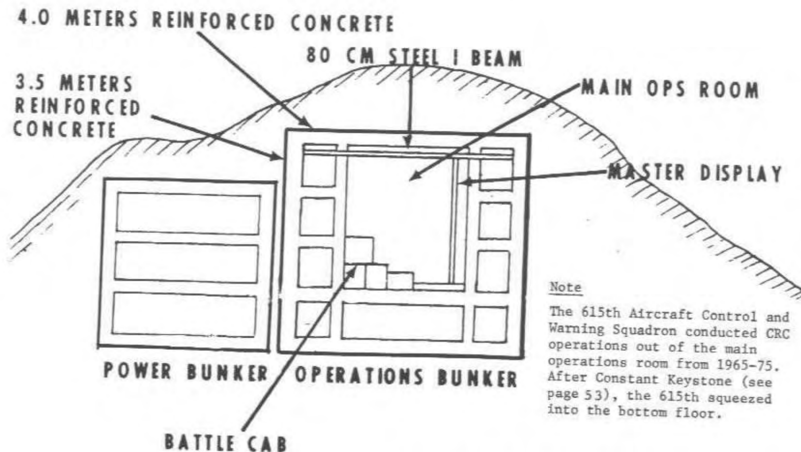
Figure IV Cutaway View of the Boerfink Bunker
