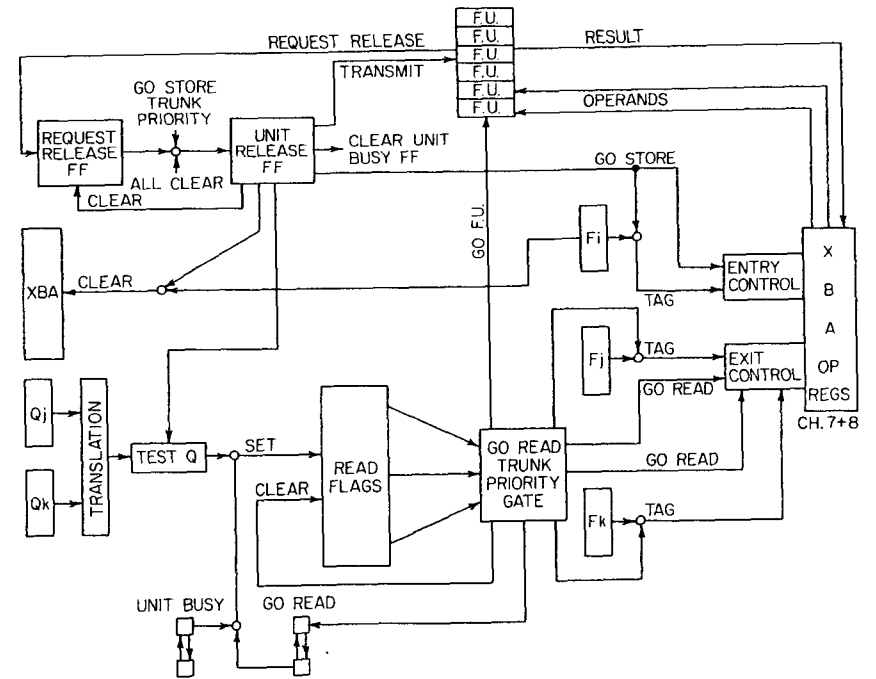
FIGURE 80 Request release block diagram.
