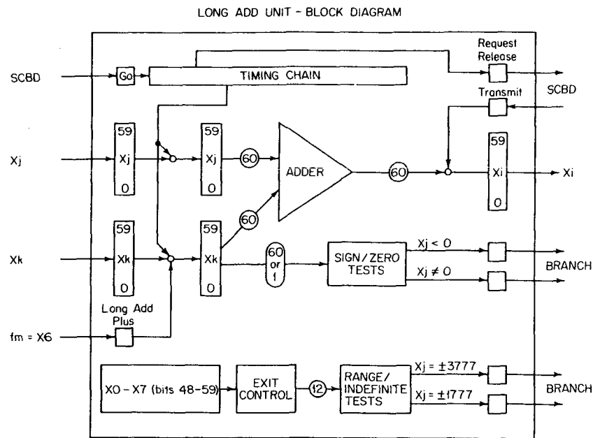
FIGURE 48 Long add unit—block diagram.
