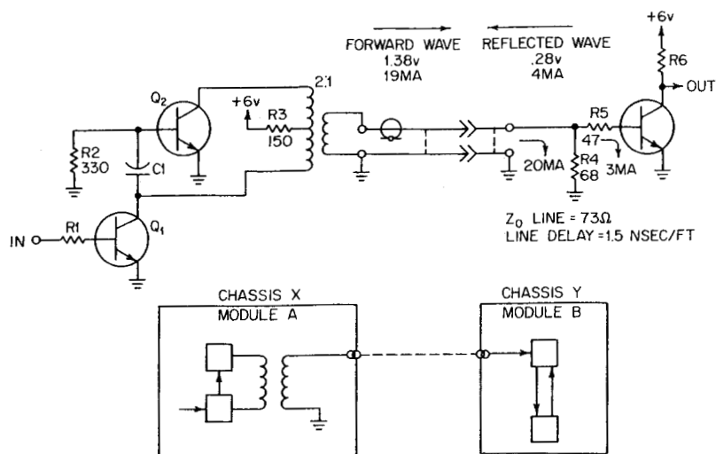
FIGURE 21 Coaxial cable driver.
