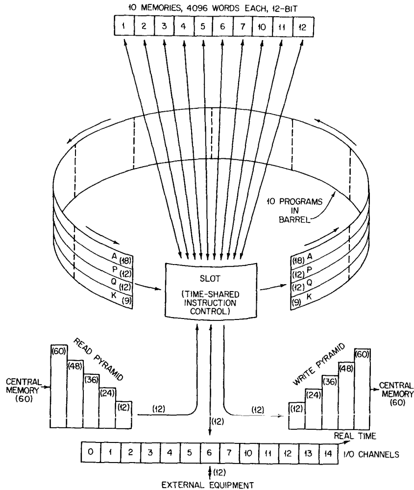
FIGURE 83 Peripheral processors.
